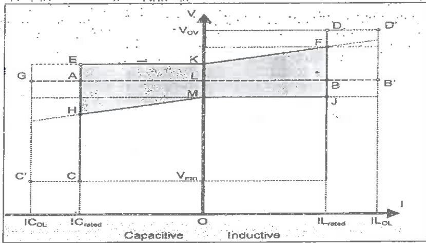
Figure-2: VI Curve of the VSC Portion
