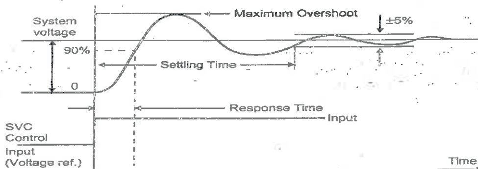
Figure-4 Response and Settling time
