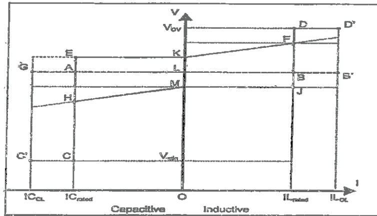
Figure-2: V-I Curve of the VSC Portion
