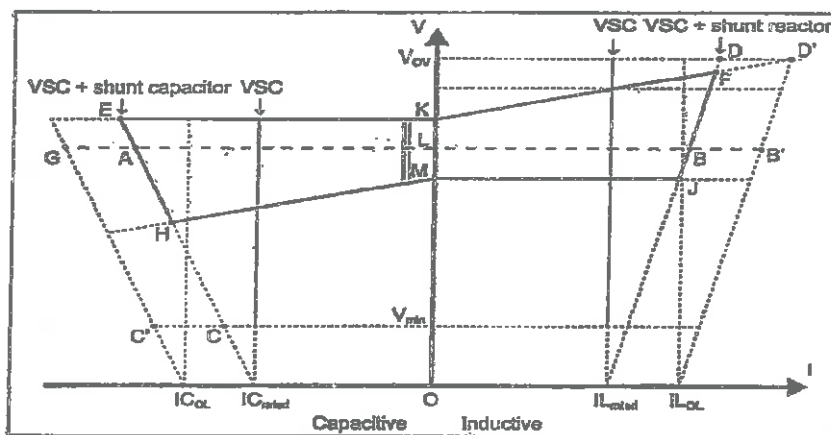
Figure-2: V-I Curve of the VSC Portion
