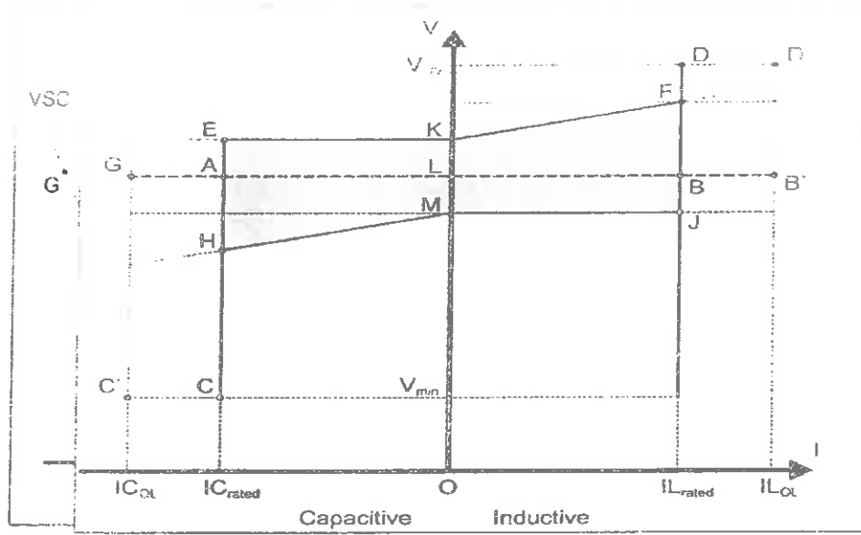
Figure-2: VI Curve of the VSC Portion
