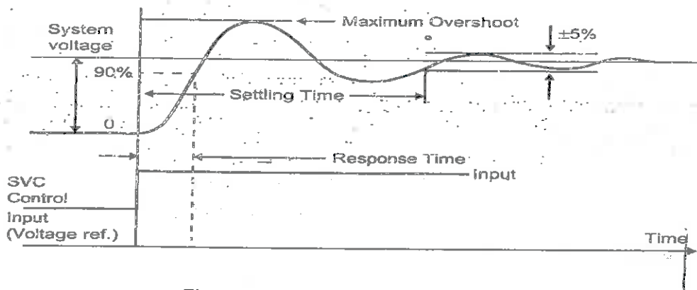
Figure-4 Response and Settling time
